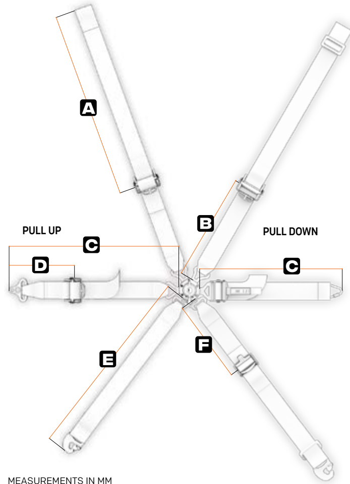
MEASUREMENTS IN MM
