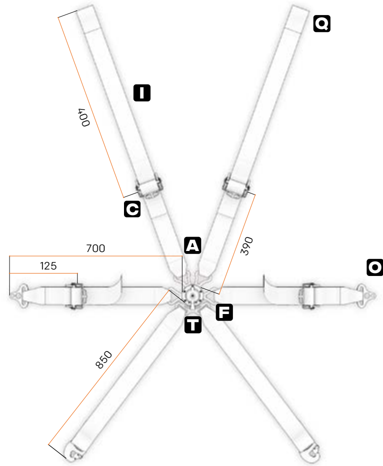
MEASUREMENTS IN MM
