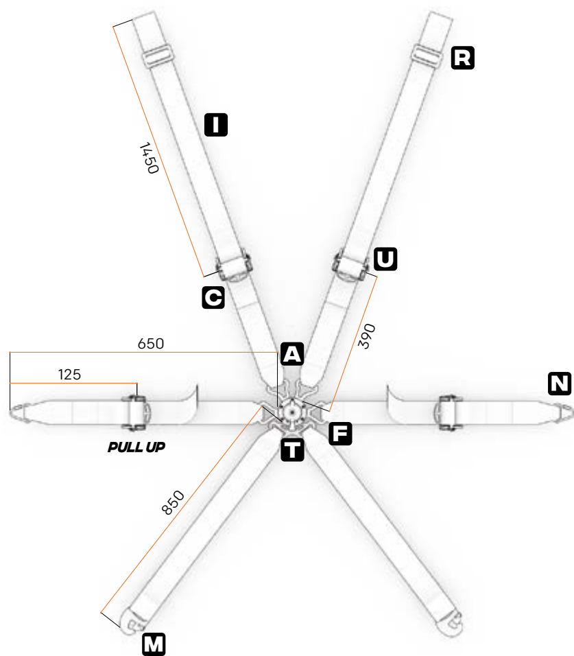
MEASUREMENTS IN MM
